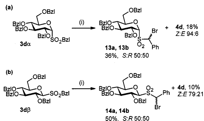
Scheme 6. Isolation of \alpha' -bromosulfones from the tandem bromination–Ramberg–Bäcklund rearrangements of 3d \alpha and 3d \beta ; (i) 0.5 g·mmol -1 KOH/Al 2 O 3 , CBr 2 F 2 , t BuOH, DCM, 5 °C
