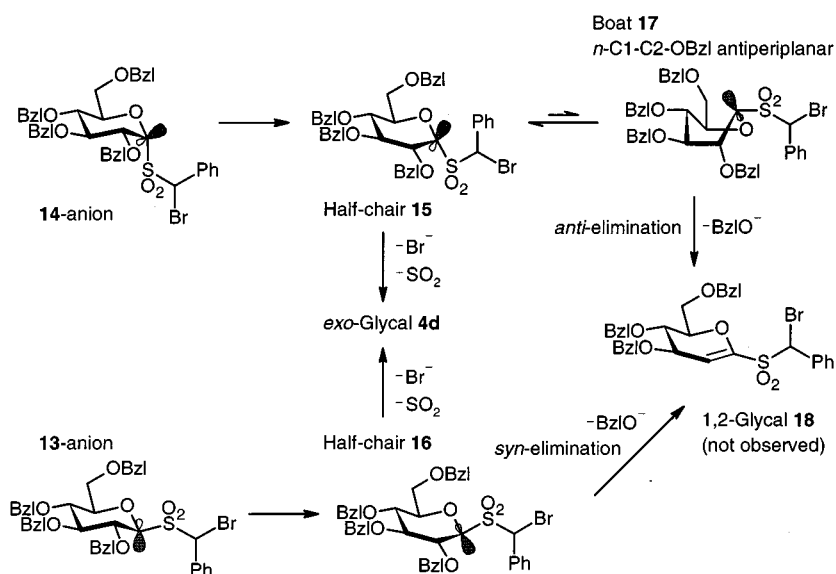
Scheme 8. Conformational requirements for 1,3- and 1,2-elimination from glycosyl \alpha' -bromosulfones leading to exo -glycals and 1,2-glycals respectively
