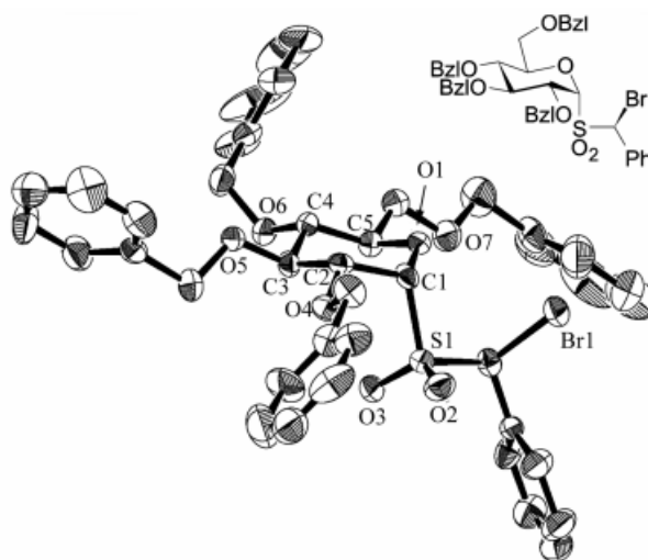
Figure 1. ORTEP representation of bromosulfone 13a
