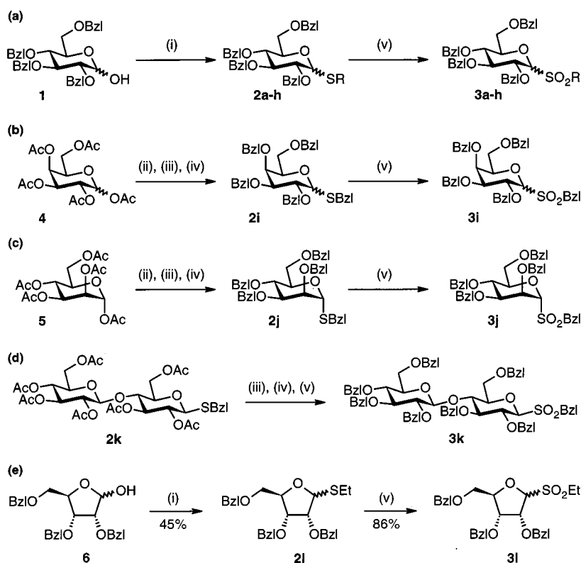
Scheme 2. (i) \text{R} \neq \text{Me} , \text{Me}_3\text{SiCl} , \text{Zn}(\text{OTf})_2 , \text{RSH} , \text{MeCN} , 40 °C; \text{R} = \text{Me} , \text{MeSSMe} , \text{BF}_3 \cdot \text{OEt}_2 , \text{MeCN} ; (ii) \text{BzSH} , \text{BF}_3 \cdot \text{OEt}_2 , \text{DCM} ; (iii) \text{MeONa} , \text{MeOH} ; (iv) \text{NaH} , \text{BzBr} , \text{DMF} ; (v) \text{R} \neq \text{CHPh}_2 , Adam, Oxone ® , acetone, \text{H}_2\text{O} , reflux; \text{R} = \text{CHPh}_2 , \text{H}_2\text{O}_2 , \text{AcOH} ; \text{R} = \text{Adam} , mCPBA, \text{NaHPO}_4 , \text{DCM} . Adam = adamant-2-yl, Bzl = benzyl; \text{DCM} = dichloromethane; mCPBA = meta -chloroperoxybenzoic acid
