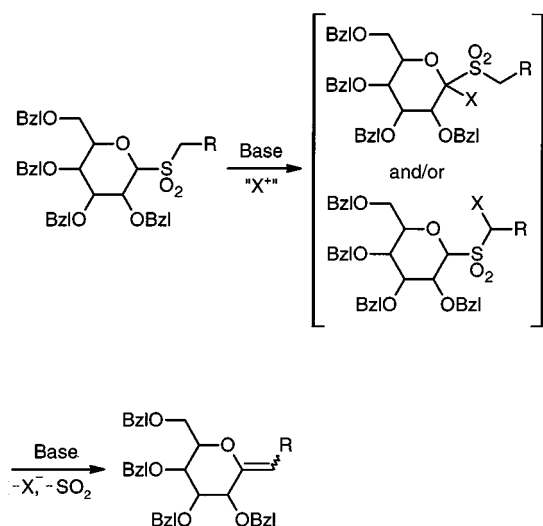
Scheme 5. Alternative pathways for the tandem halogenation–Ramberg–Bäcklund rearrangement of glycosyl sulfones involving regioisomeric halosulfones
