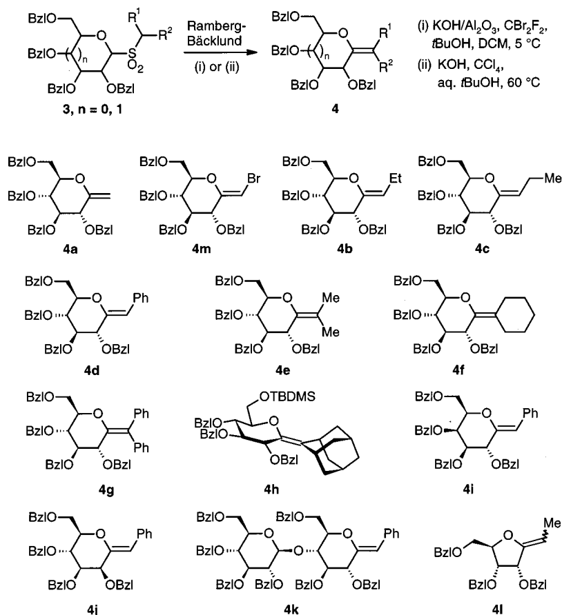
Scheme 3. The scope of the Ramberg–Bäcklund rearrangement of glycosyl sulfones
