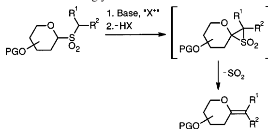
Scheme 1. Generic representation of the transformation of glycosyl sulfones into exo -glycals via a Ramberg–Bäcklund rearrangement. PG = protecting group
