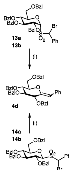
Scheme 7. (i) 7.5 g·mmol -1 KOH/Al 2 O 3 , t BuOH, DCM, 5 °C; see Table 3 for yields
